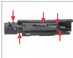
Lubricate the bolt at the points shown.
