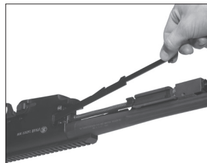
Pull the action bars forward and out of the receiver.
