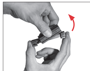
Compress the springs and separate the inertia block.
