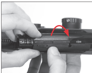
Carefully rotate the bolt out of the receiver.
