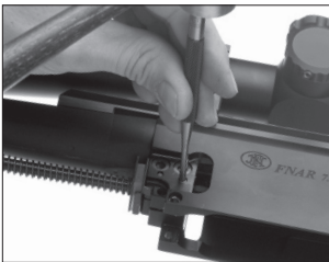
Tap out the pin from the left to the right side.
